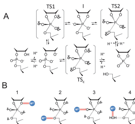
Fig. 1 (A) Mechanisms of RNA 2'-O-transphosphorylation. Specific base catalysis involves equilibrium deprotonation of the 2'O resulting in a 2'O oxyanion that acts as a nucleophile attacking the adjacent phosphoryl group. Experimental and computational data support a mechanism that involves a late TS (similar to TS2). Acid catalysis proceeds via a stepwise mechanism shown in the top pathway resulting in the formation of a stable phosphorane intermediate. The intermediate shown here is anionic for simplicity, however, in the acid mechanism this intermediate is protonated on one or more of the non-bridging oxygens. The potential formation of 2',5' diester products resulting from isomerization are also omitted for clarity. (B) Proposed metal ion catalytic modes involving interactions with anionic TSs for RNA cleavage. Potential modes include interactions with the 2'O nucleophile (1), 5'O leaving group (2), and non-bridging oxygen (3). These interactions can involve direct coordination (1–3), H-bonding or transfer (4).
