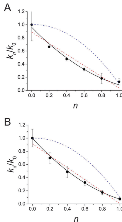
Fig. 2 Proton inventory of specific base (A) and Zn 2+ -catalyzed (B) RNA 2'-O-transphosphorylation. The data are fit to a linear function or to the Gross-Butler equation (eqn S3, ESI†). The red dashed line represents a model for one normal fractionation factor of ( \varphi^T = 0.14 ). The blue dashed line a simulation using eqn S3 (ESI†) for a model involving acid catalysis in which there is a modest inverse fractionation factor ( \varphi^R = 2 ) due to an increase in the protonated form of the catalyst at constant pH that necessitates a large offsetting normal fractionation factor ( \varphi^T = 0.05 ). The solid black line assumes two normal fractionation factors: one reflecting the change in pK_a of the 2'-OL ( 1/\varphi^R = 0.2 ) and a second normal contribution of \varphi^T = 0.4 .
