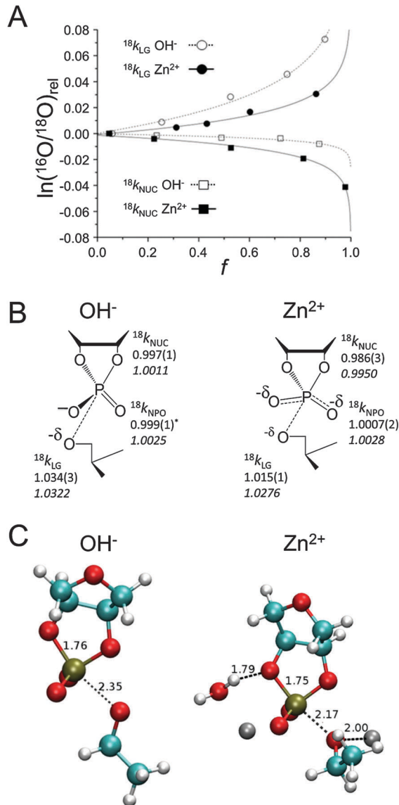
Fig. 3 Summary of KIE measurements for catalysis by specific base ( \text{OH}^- ) and \text{Zn}(\text{II}) . (A) Determination of ^{18}k values by fitting the \ln(^{18}\text{O}/^{16}\text{O})_{\text{rel}} in the unreacted substrate as a function of reaction progress ( f ) to eqn S4 (ESI†). (B) Summary of observed ^{18}k_{\text{NUC}} , ^{18}k_{\text{NPO}} and ^{18}k_{\text{LG}} values. Standard errors in the last numeral are shown in parentheses. The KIEs predicted from the TS models in part C are shown in italics. (C) TS models from DFT calculations for specific base catalysis and a model \text{Zn}^{2+} -catalyzed mechanism from Chen et al. Distances along the reaction coordinate for the 2′O–P bond formation and 5′O–P bond cleavage are indicated in angstroms. A two metal ion model for non-enzymatic catalysis by \text{Zn}^{2+} . As described in the text a two metal ion mechanism in which a metal ion interacts with the 5′O leaving group ( M_{\text{A}} ) and a second metal ion interacts via coordination to a non-bridging oxygen and via H-bonding to the 2′O ( M_{\text{B}} ).
